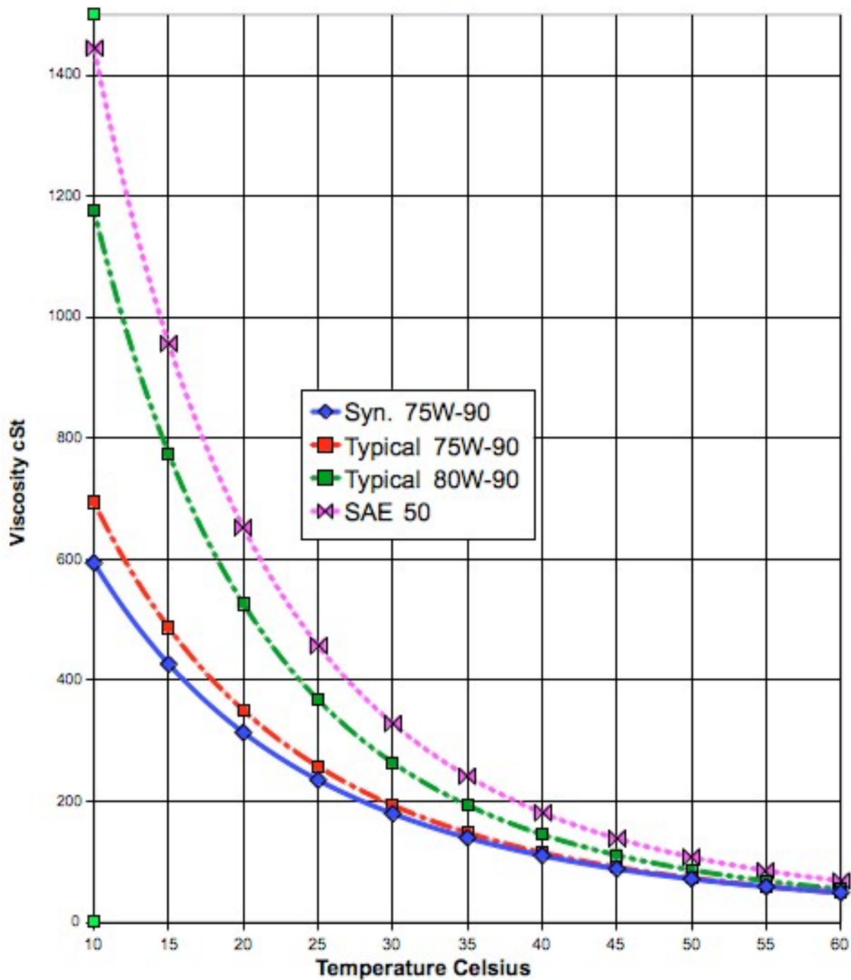
Viscosity Curve
